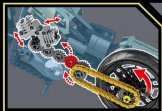
CYLINDER GEAR DRIVE 汽缸齿轮传动
